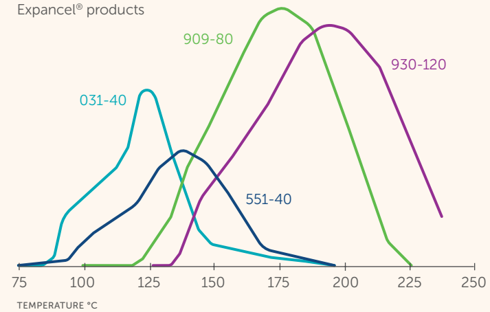
Expansion curves for several Expancel® products
